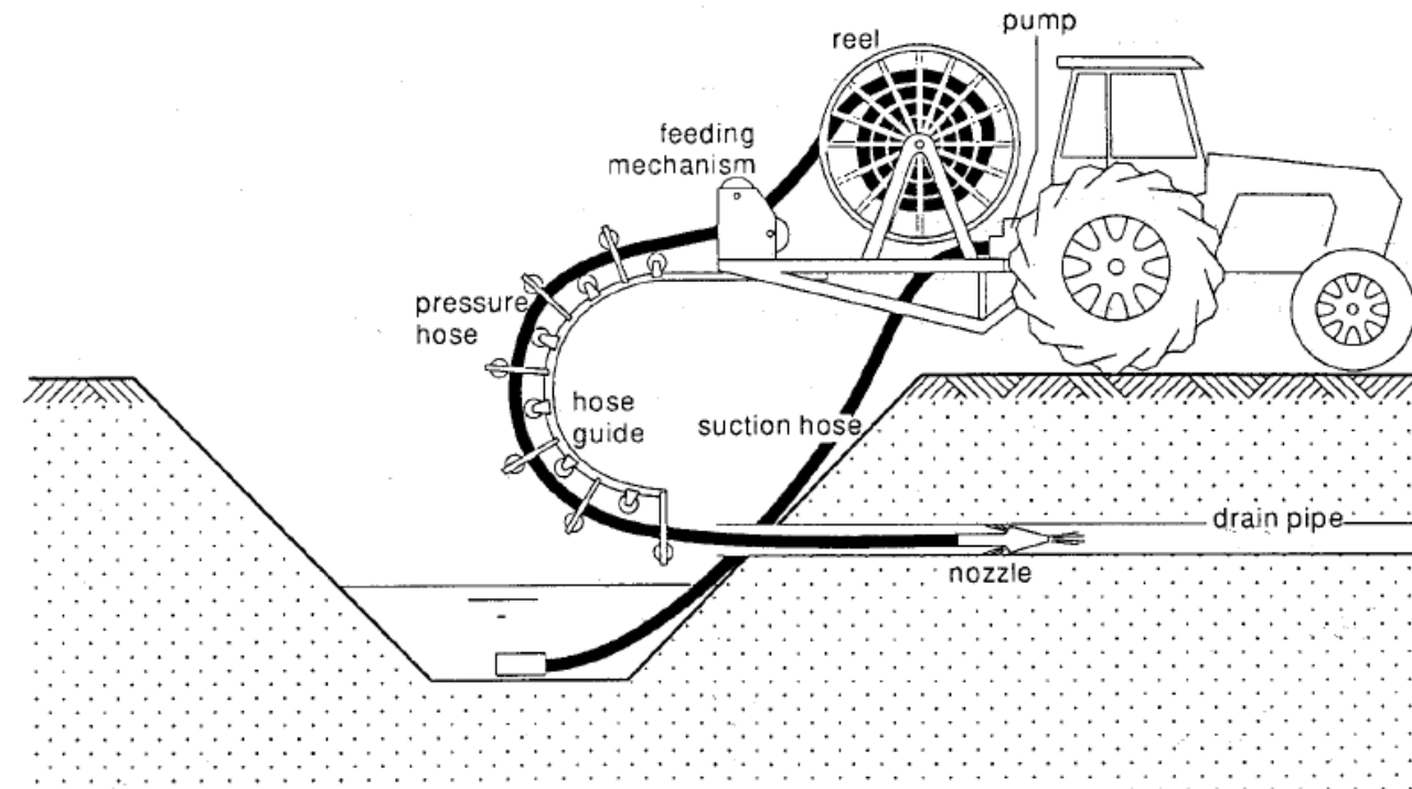
High-pressure purging machine
